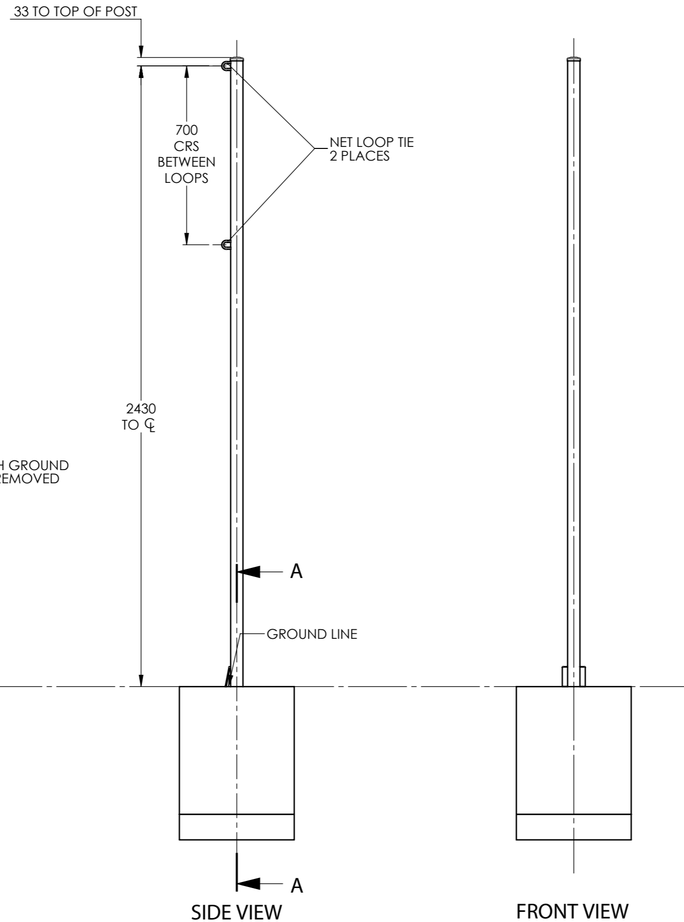
(ALSO AVAILABLE VP02 60mmOD POST) CMA VP01 STANDARD REMOVABLE VOLLEYBALL POST
